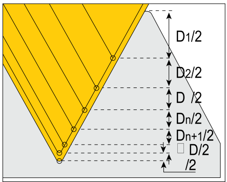
Flank diminishing
