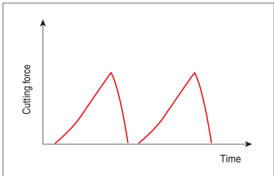
Straight flute
