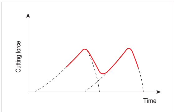
Helix flute
