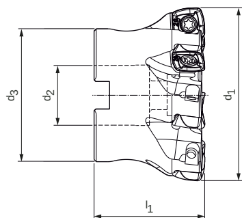
Milling cutter head
