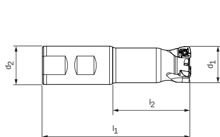
End milling cutter
