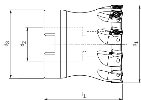
Milling cutter head
