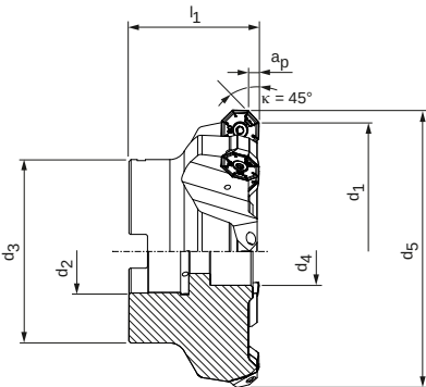
Milling cutter head, close spacing
