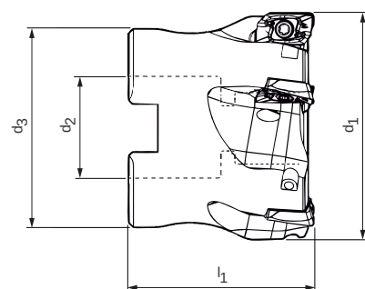
Milling cutter head
