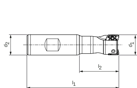
End milling cutter
