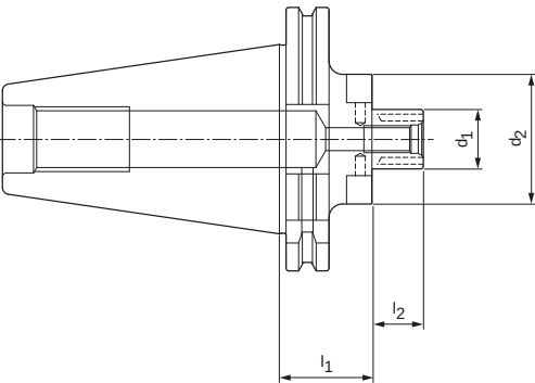
SK shank with decentralised coolant delivery
